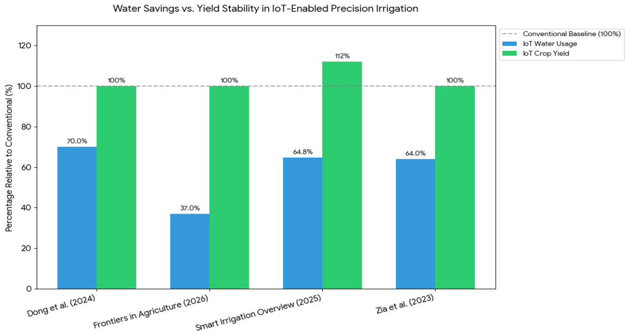
Fig. 1: Chart visualizing the performance of IoT systems across four key studies, using conventional methods (set as 100%) as the baseline.
