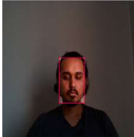
Figure 1. Classes annotation.
