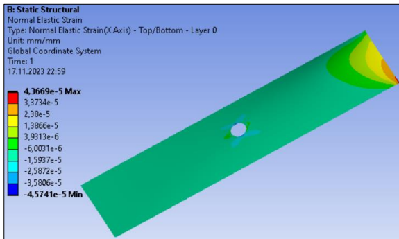
c) Normal elastik strain.
