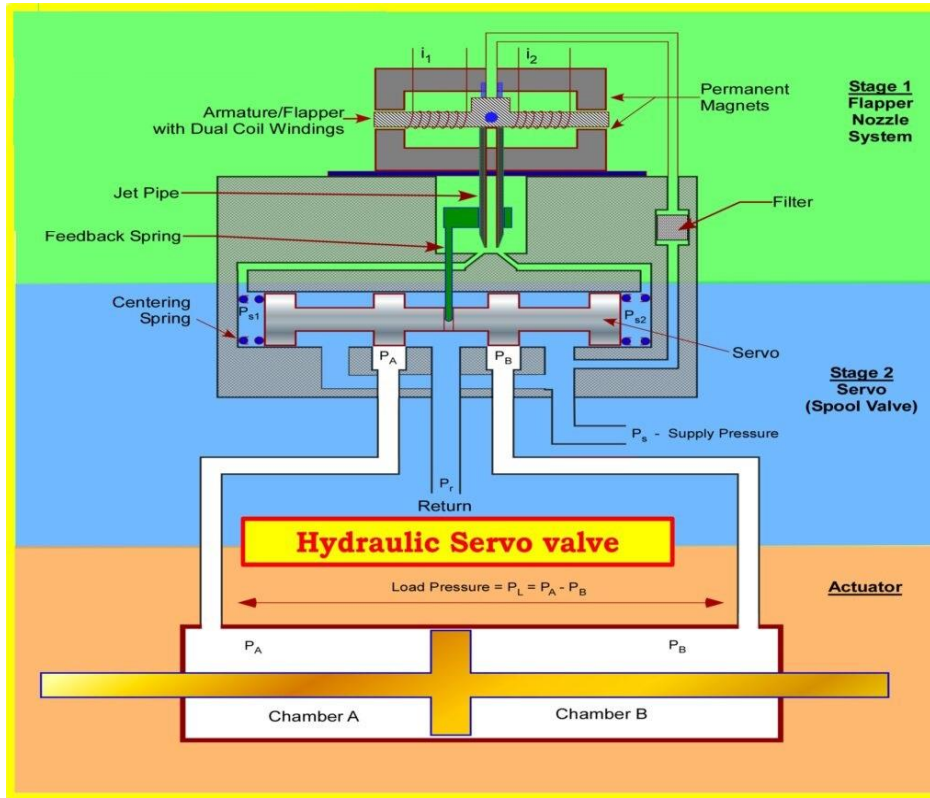
Figure 2. Hydraulic servo valve working principle schematic illustration (Automationforum.com, 2023; DesignAerospace LLC, 2013).
