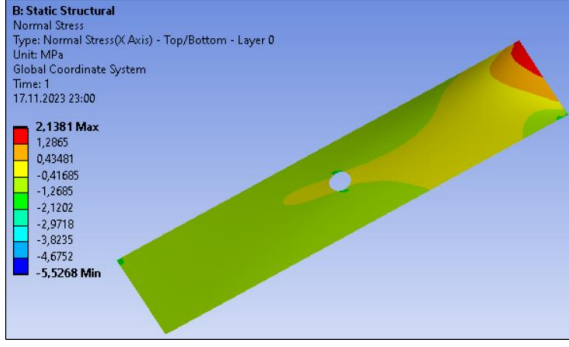
e) Normal Stress.
