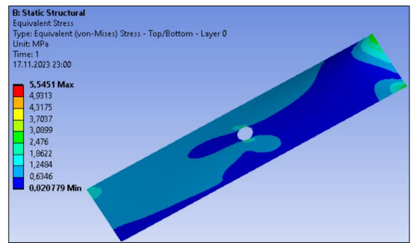
d) Equivalent Stress.
